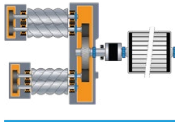
"Oil-Free" Screw Compressor
