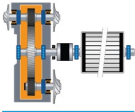
Traditional Turbo Compressor
